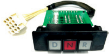
ZF 3 Button Gear Selector Horizontal/Vertical Round
